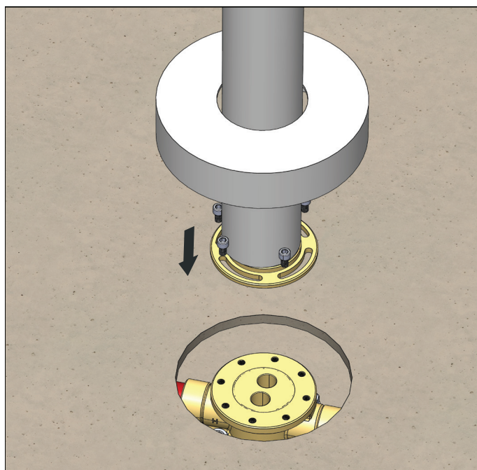
Insert trim onto valve. Tighten screws
