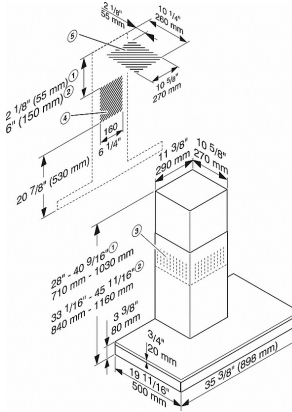
DA 6698 W, CLST (Installation drawing) - USA
