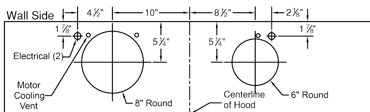
900 CFM B200 Dual &amp; B100 Single Blower (Top View)
