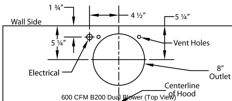
CONNECTION DIAGRAM
