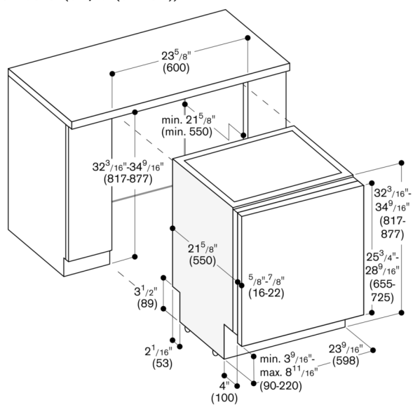
Connection dimensions for a 24" (600 mm) wide dishwasher
