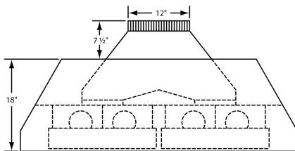
1200 CFM Double B200 Dual Blowers (Top View)
