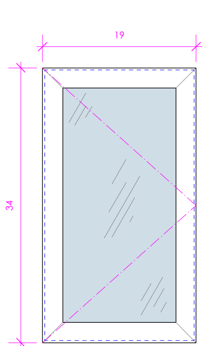
18-1/2" w x 33-1/2" CUTOUT FOR RECESSED INSTALLATION
