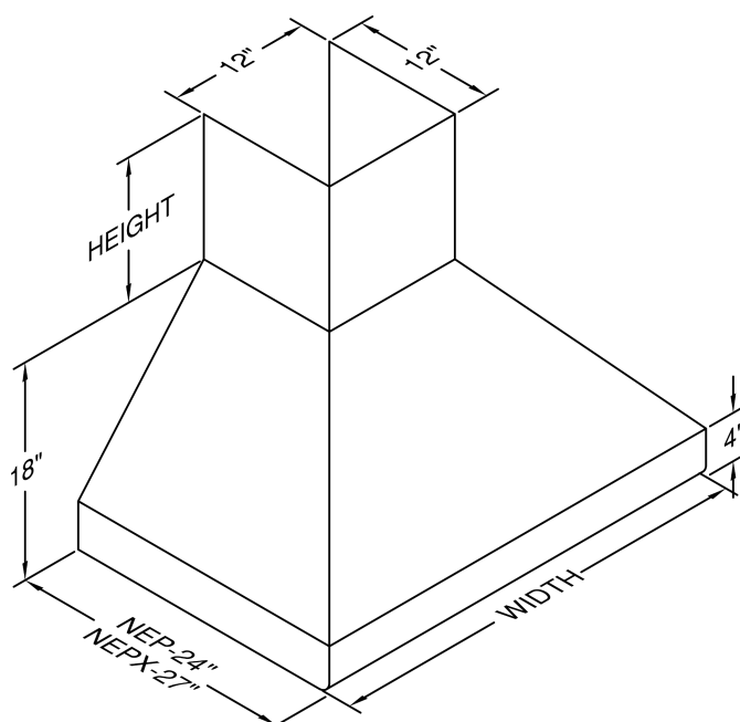
CONNECTION DIAGRAM
