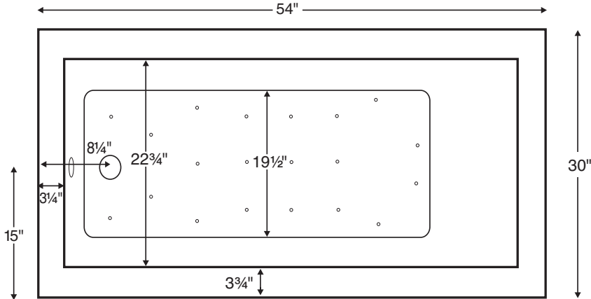
The Sculpted Finish process does not allow enough space for mounting fixtures on the tub deck. Shown as Air Bath
