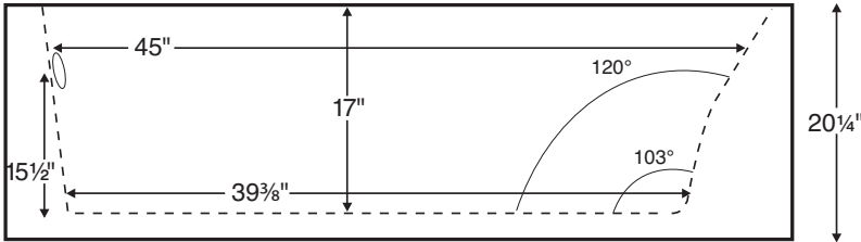
The Sculpted Finish process does not allow enough space for mounting fixtures on the tub deck. Shown as Air Bath
